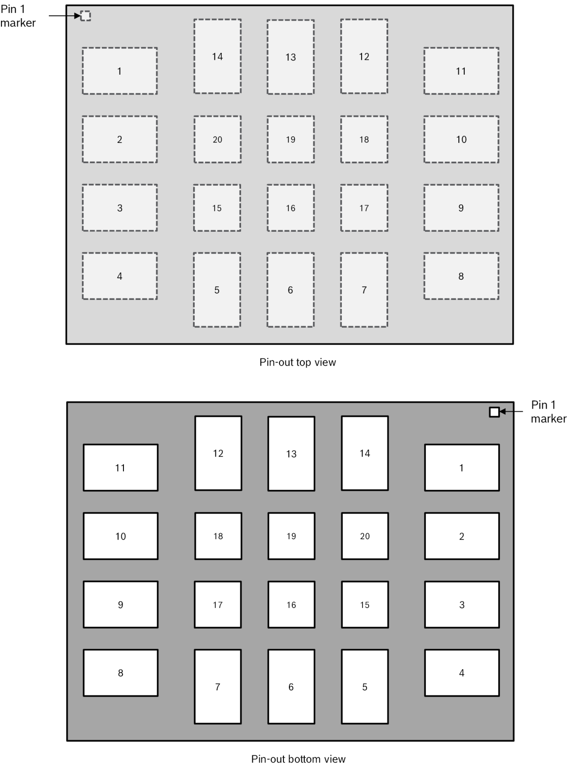
Figure 2 : Pad Connections
