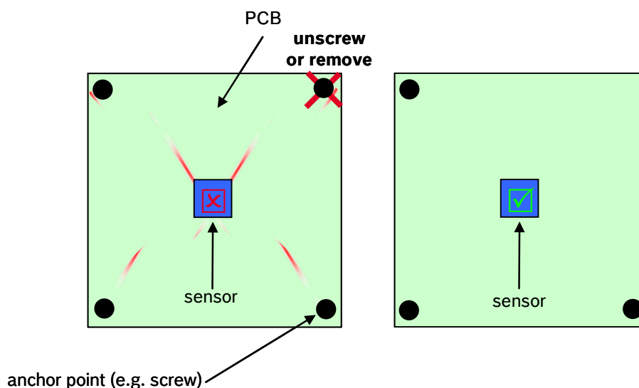
Figure 5: redundant PCB anchor points
