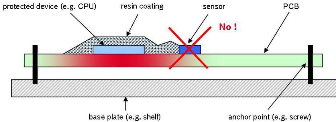
Figure 7: Resin coatings
