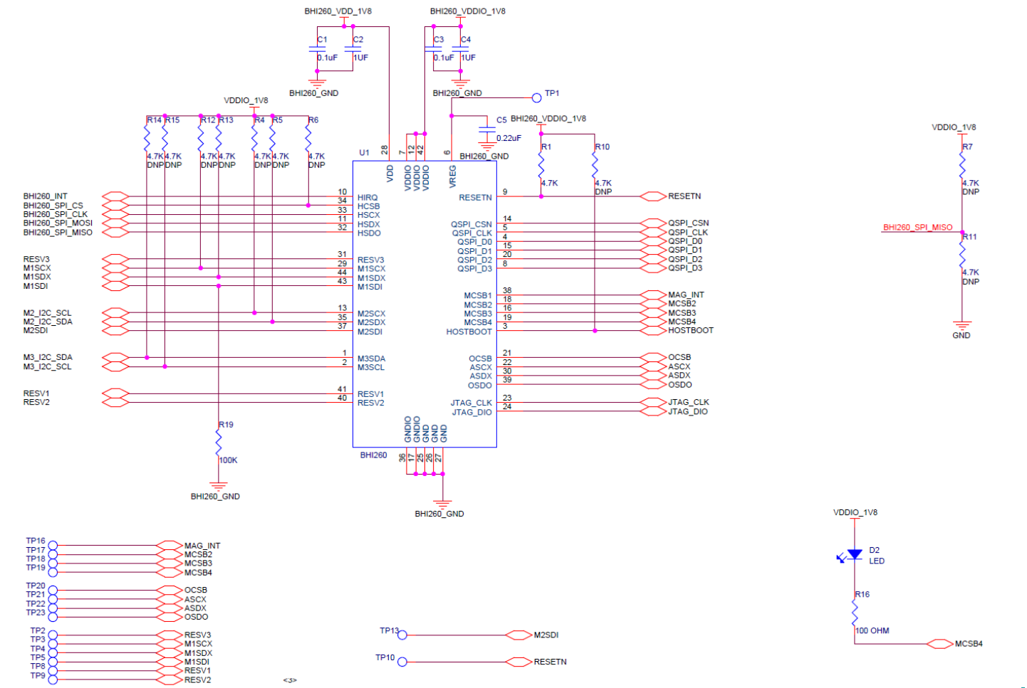
BHI260AB shuttle board schematics
